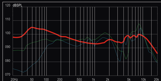
H30 Frequency Response Curve
